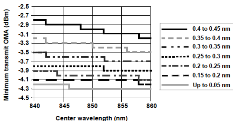
Gambar 2. 10GBASE-S minimum transmit power (IEEE 802.3-2008)
